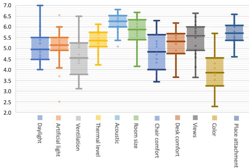
Figure 2. iPEP boxplot.
